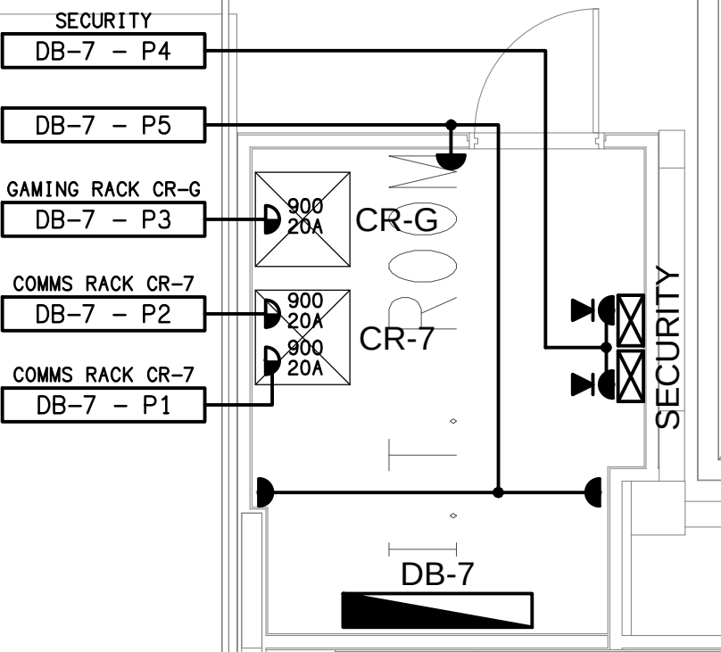
DETAIL A IT ROOM FLOOR PLAN SCALE 1:50
